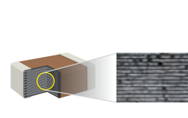
Thick-film process technology Printing and multilayering electrodes and other elements to produce chip capacitors, chip inductors, and other layered electronic components.
